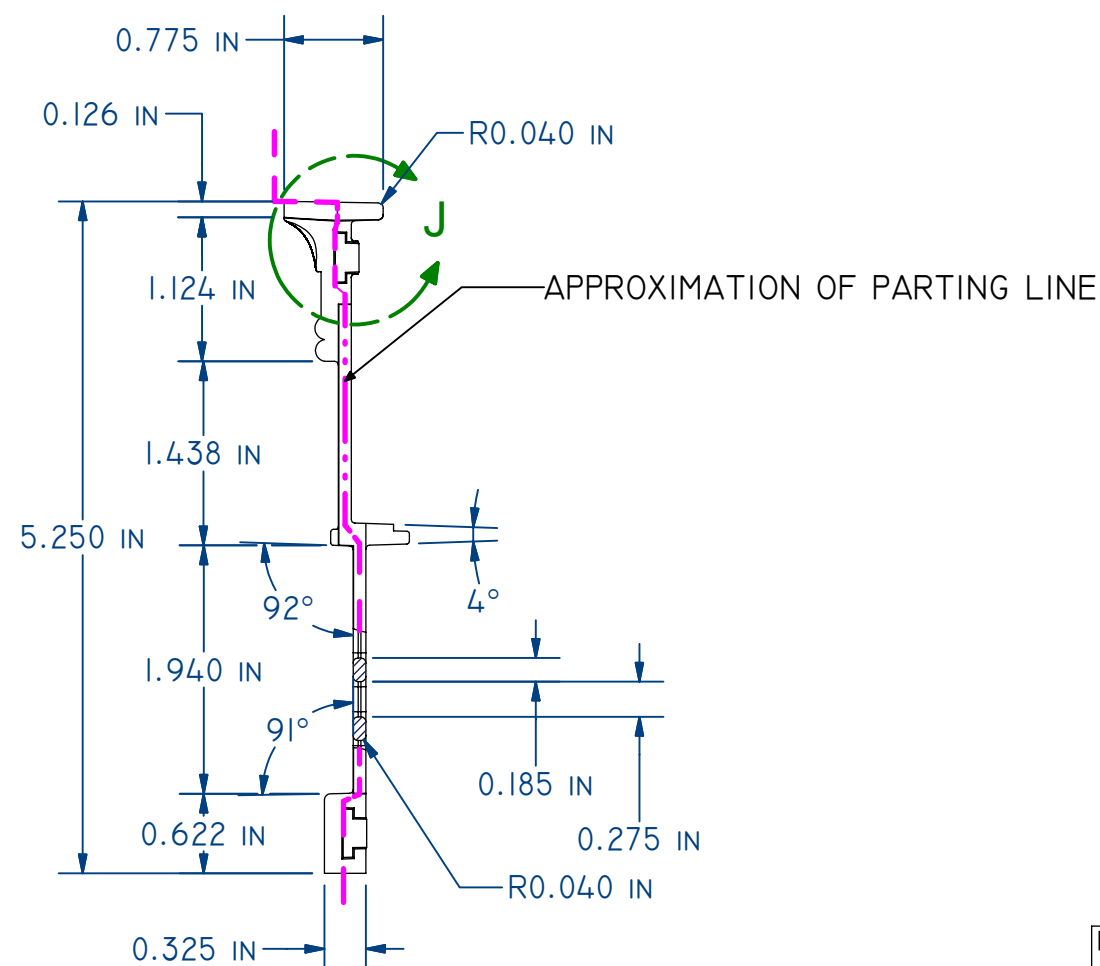
DETAIL K SCALE 1 : 1
