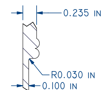
DETAIL K SCALE 1 : 1
